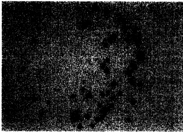
Fig. 3. Example of colony blot hybridization of V. vulnificus from raw oysters.
