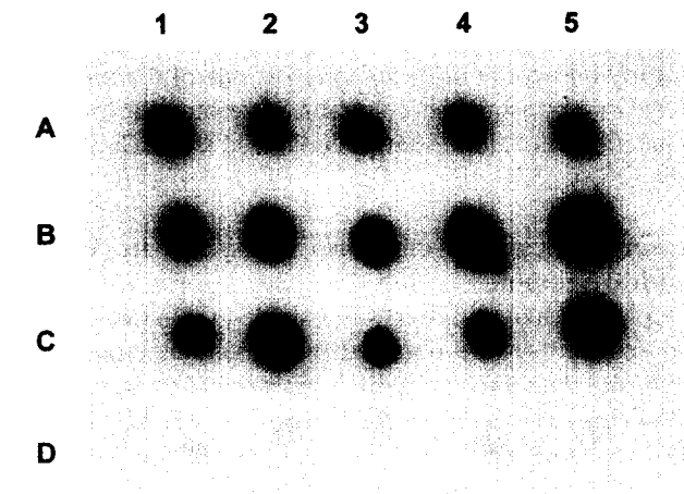
Fig. 1. Colony blot hybridization of Vibrio spp. with ^{32}\text{P} -labeled vvhA DNA probe.
