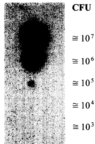
Fig. 2. Analysis of the limit of V. vulnificus detection using dot blot hybridization with ^{32}\text{P} -labeled vvhA DNA.
